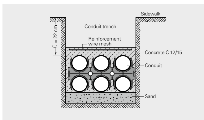
Protection of the conduit layer against deflection and mechanical damage when going below the minimum cover (example see also KRV A 515).
