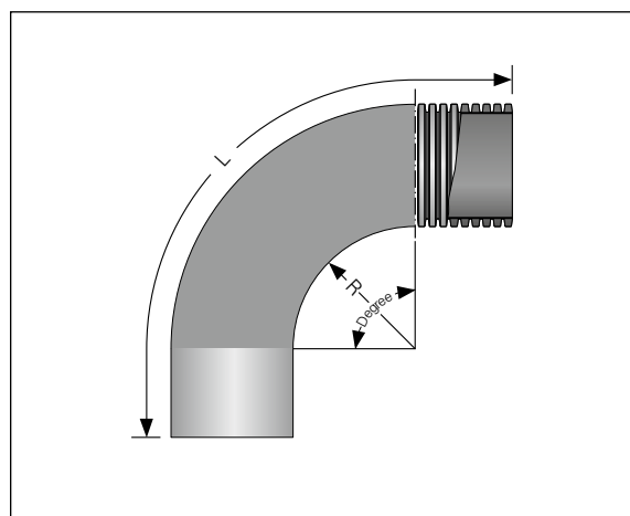
Nominal diameter and radius R of the conduit bend (inside of bend)
