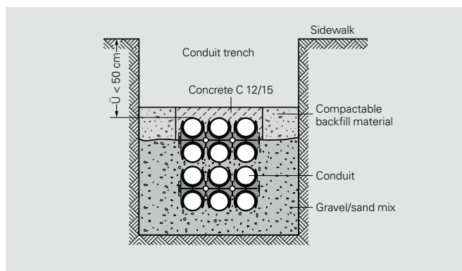
Conduit layer installed in concrete with minimum cover (example see also KRV A 515/A 535).
