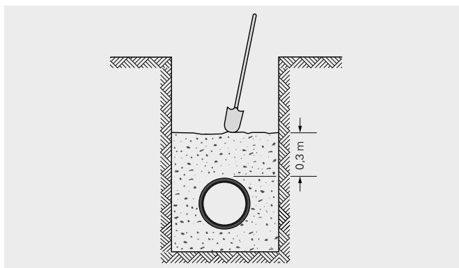
Backfill and compact conduit up to 30 cm above the conduit crown by hand with stoneless, compactable soil.
